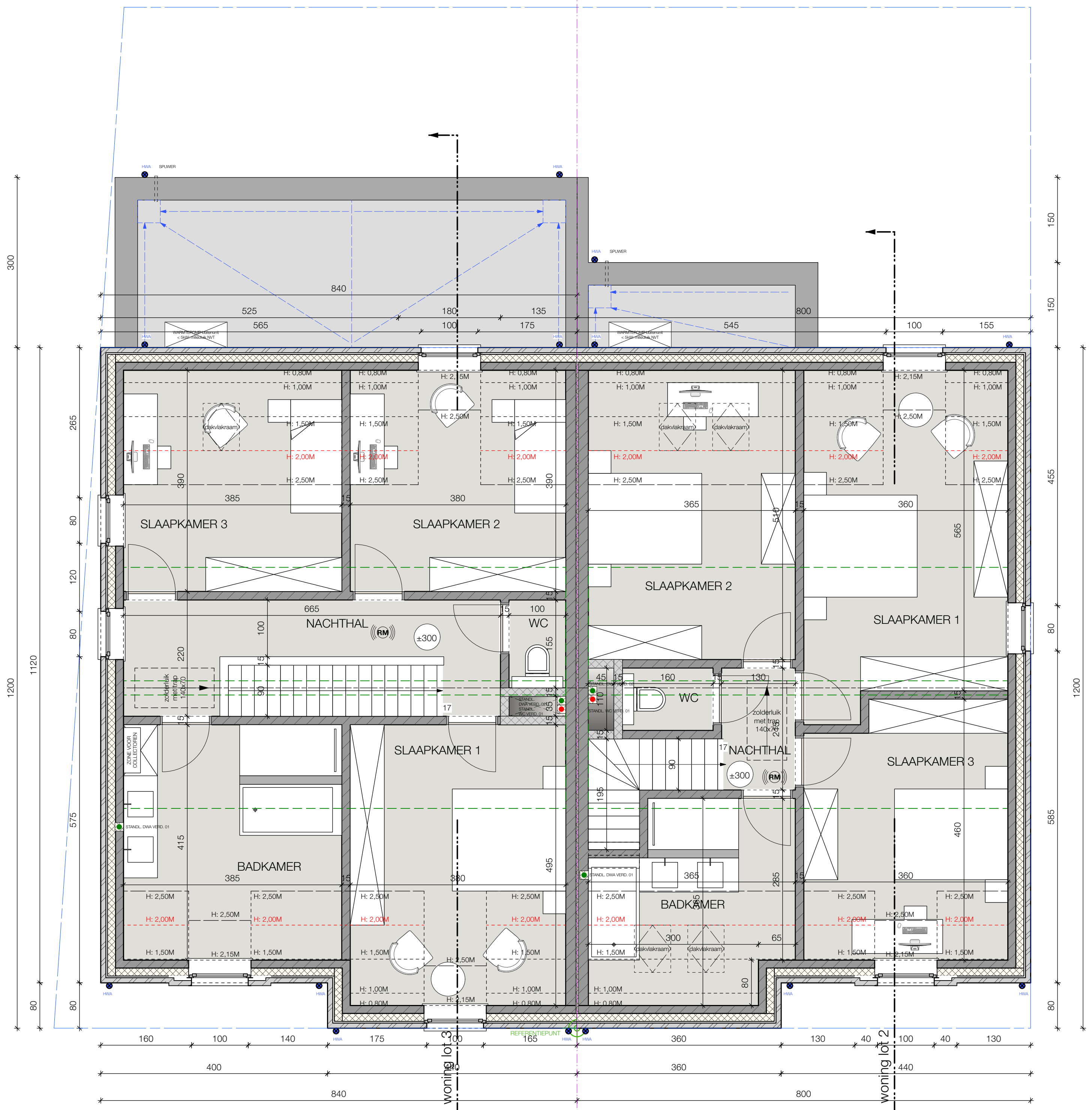
PLAN 01 bebouwd opp. ±97,60m 2 LOT 3
