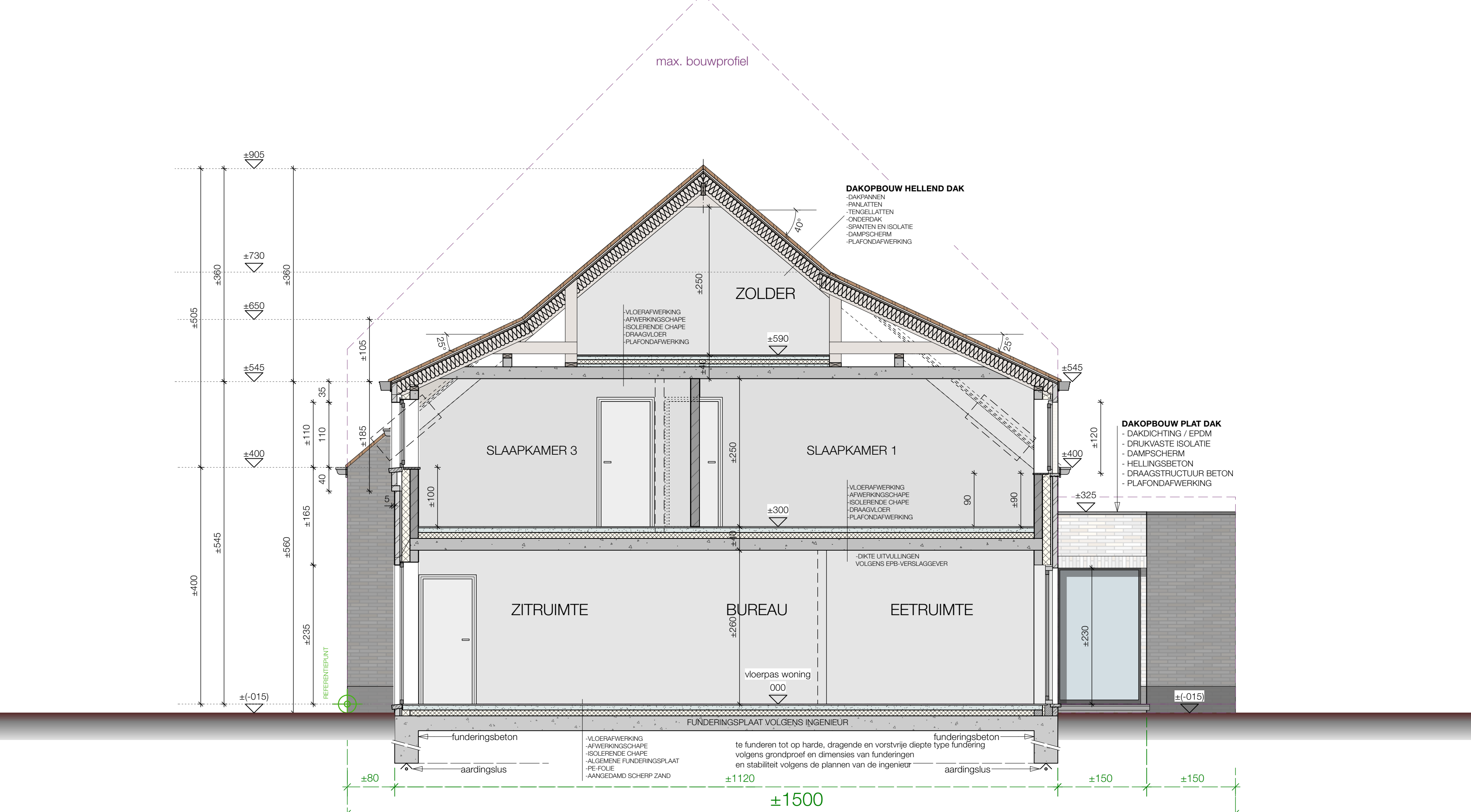
LOT 2 DOORSNEDE woning 2
