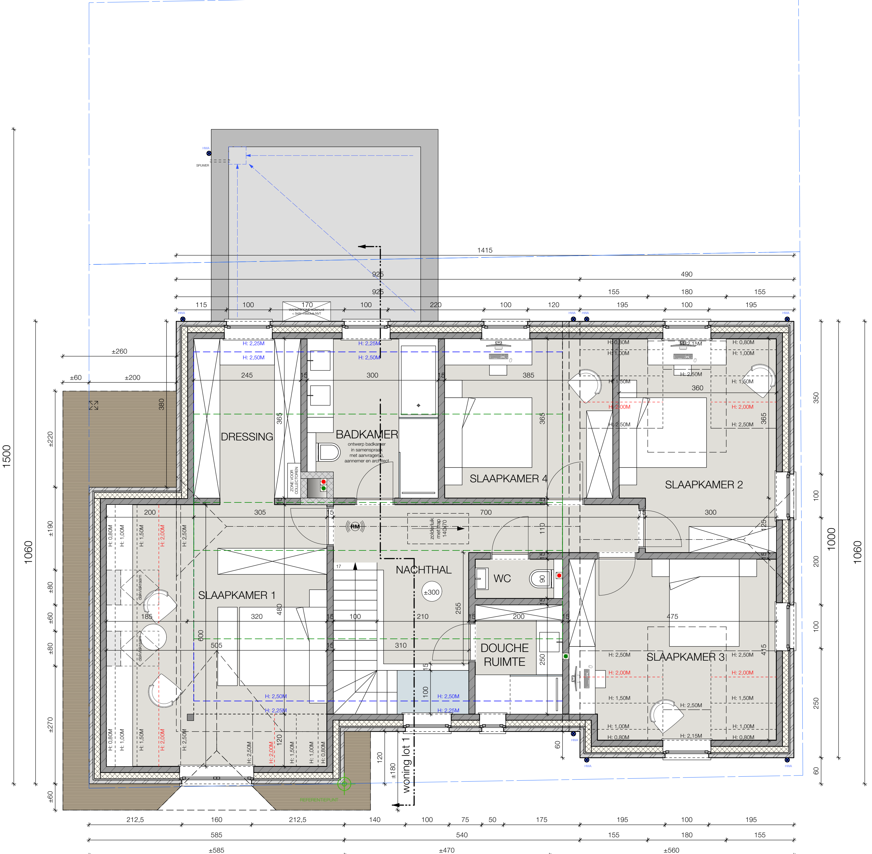
PLAN 01 bebouwd opp. ±154,17m 2 LOT 1
